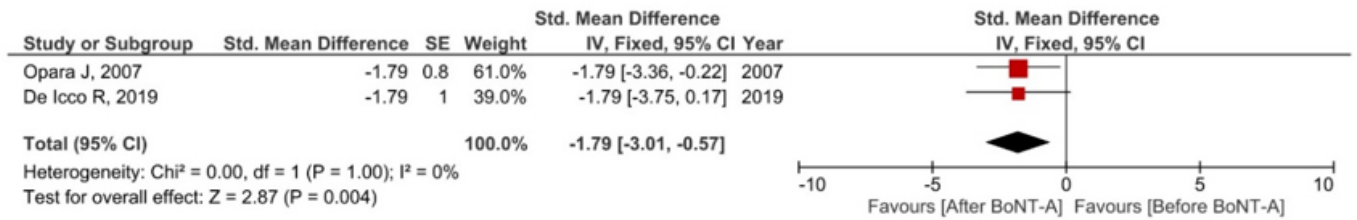
Supplementary Fig. S4. When correlation coefficient=0.00. Forest plot comparing the changes in the pain score between before botulinum toxin-A (BoNT-A) and after BoNT-A treatment in spinal cord injury. 95% CI, 95% confidence interval; SE, standard error; IV, independent variable.
