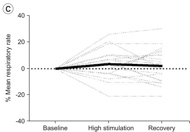
Supplementary Fig. S8. The response of mean respiratory rate in (A) sham, (B) continuous low-amplitude, (C) continuous high-amplitude, and (D) pulsed stimulations. Bold solid lines represent average values and dotted lines represent individual values.
