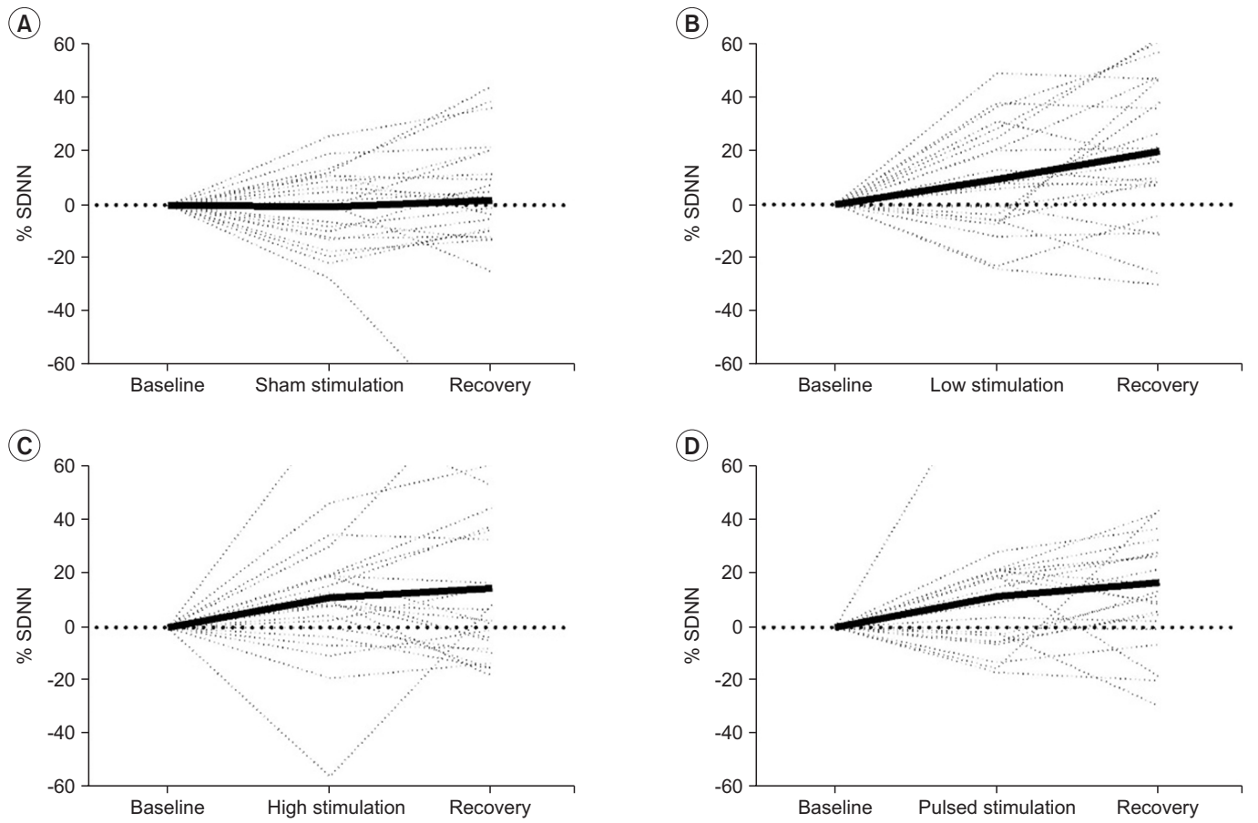
Supplementary Fig. S2. The response of standard deviation of R-R intervals (SDNN) in (A) sham, (B) continuous low-amplitude, (C) continuous high-amplitude, and (D) pulsed stimulations. Bold solid lines represent average values and dotted lines represent individual values.
